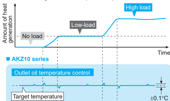
Note: Pattern diagram with the heating load stabilized at 0 - 100%
