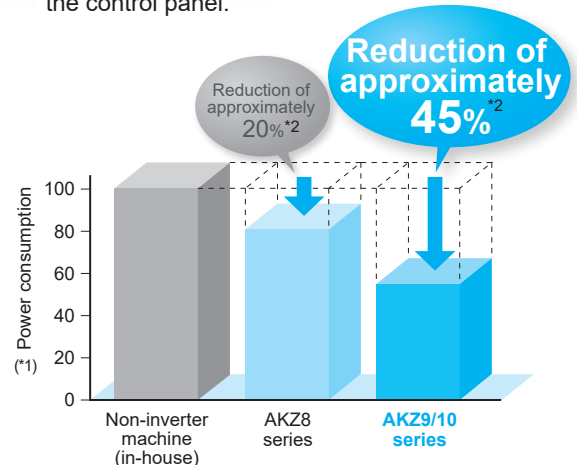
Note: Pattern diagram with the heating load stabilized at 0 - 100%
